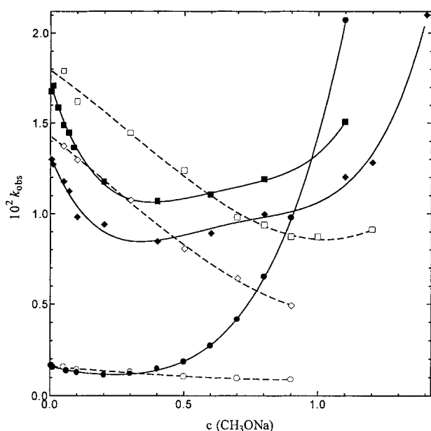
Figure 1. Dependence of observed rate constants k_{\text{obs}} (s -1 ) of methanolysis of 1-acyl-3-(2-halo-5-nitrophenyl)thioureas 1a (squares) c (diamonds) and d (circles) in sodium methoxide solution (concentration in mol l -1 ), without addition (solid symbols) and with addition (open symbols) of 18-crown-6. The curves represent only the nature of the dependence
