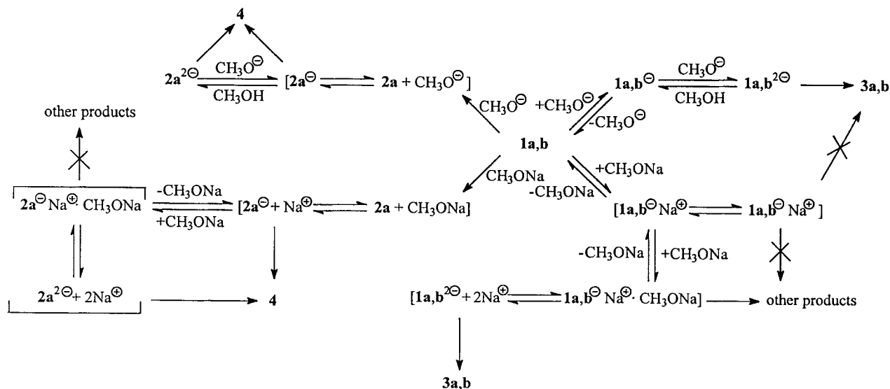
Scheme 3. (a) Upper part of the scheme is in the presence of 18-crown-6. (b) CH 3 ONa is the sum of solvated ions and ion pair. (c) 1a, b - means anions of 1a, b and similarly for other anions. (d) We have no idea about the mechanism of formation of other products but from the steep increase in K_{\text{obs}} of 1c and d with increase in concentration of sodium methoxide (Fig. 1) we suggest that there are two sodium cations in the activated complex of the rate-limiting step. 1a - Na + · CH 3 ONa is the possible structure of the encounter complex, and similarly for 2a - Na + · CH 3 ONa
